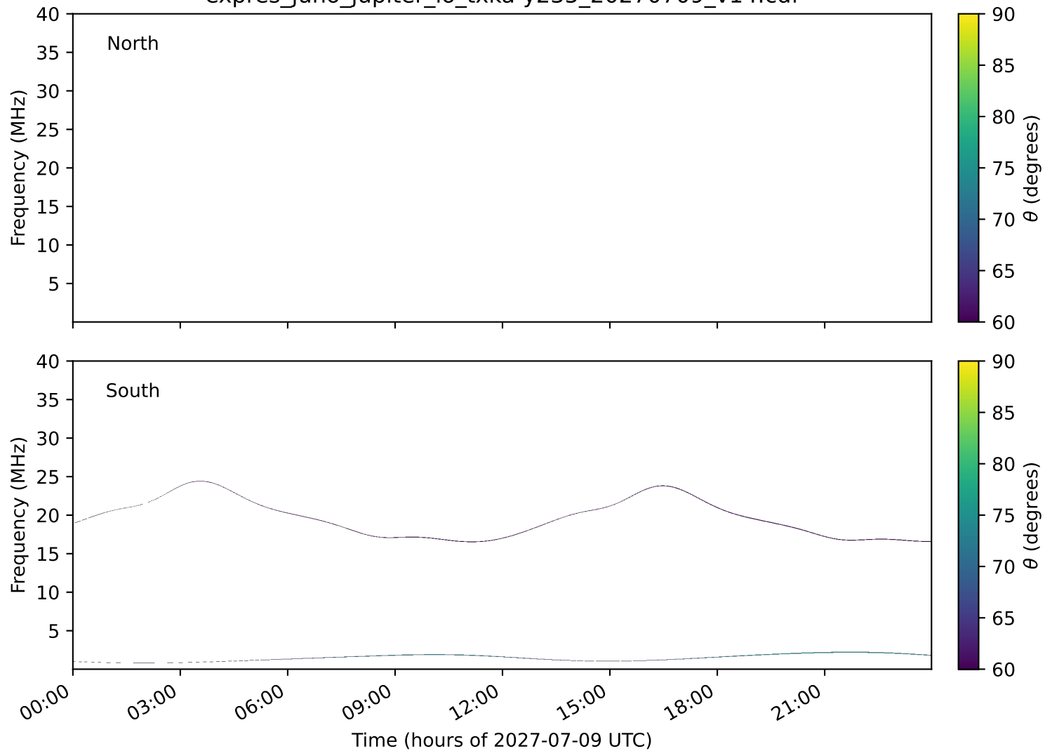
expres_juno_jupiter_io_txka-y235_20270709_v14.cdf
