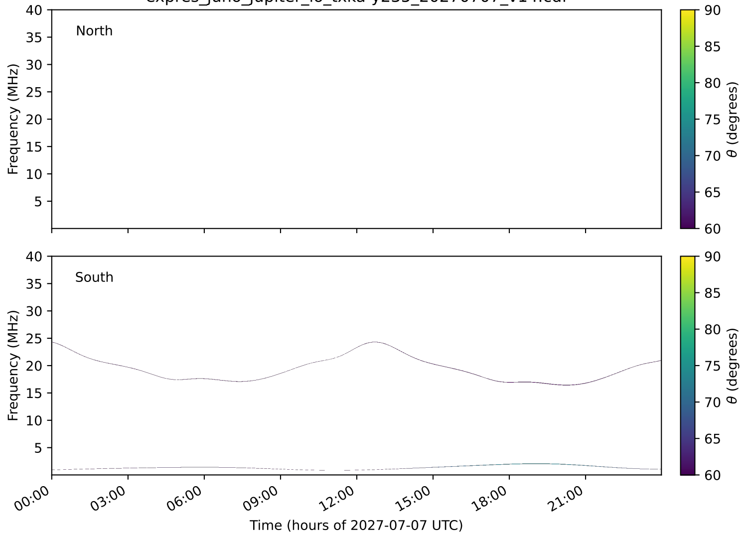
expres_juno_jupiter_io_txka-y235_20270707_v14.cdf
