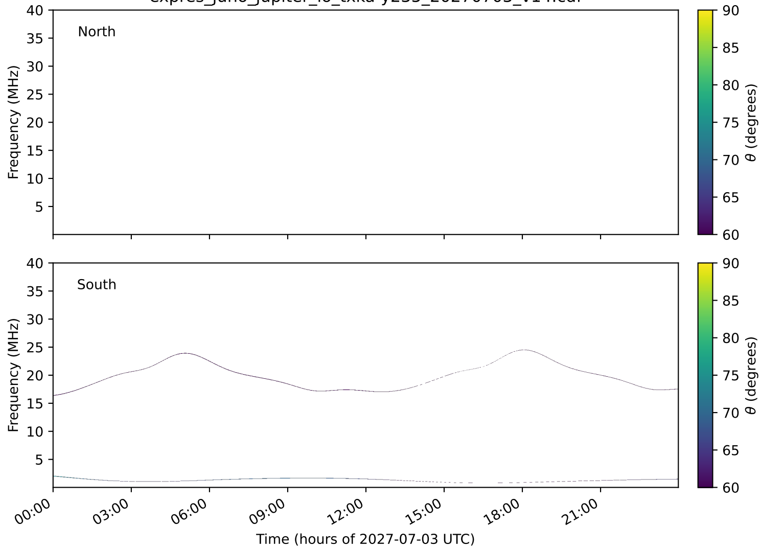
expres_juno_jupiter_io_txka-y235_20270703_v14.cdf
