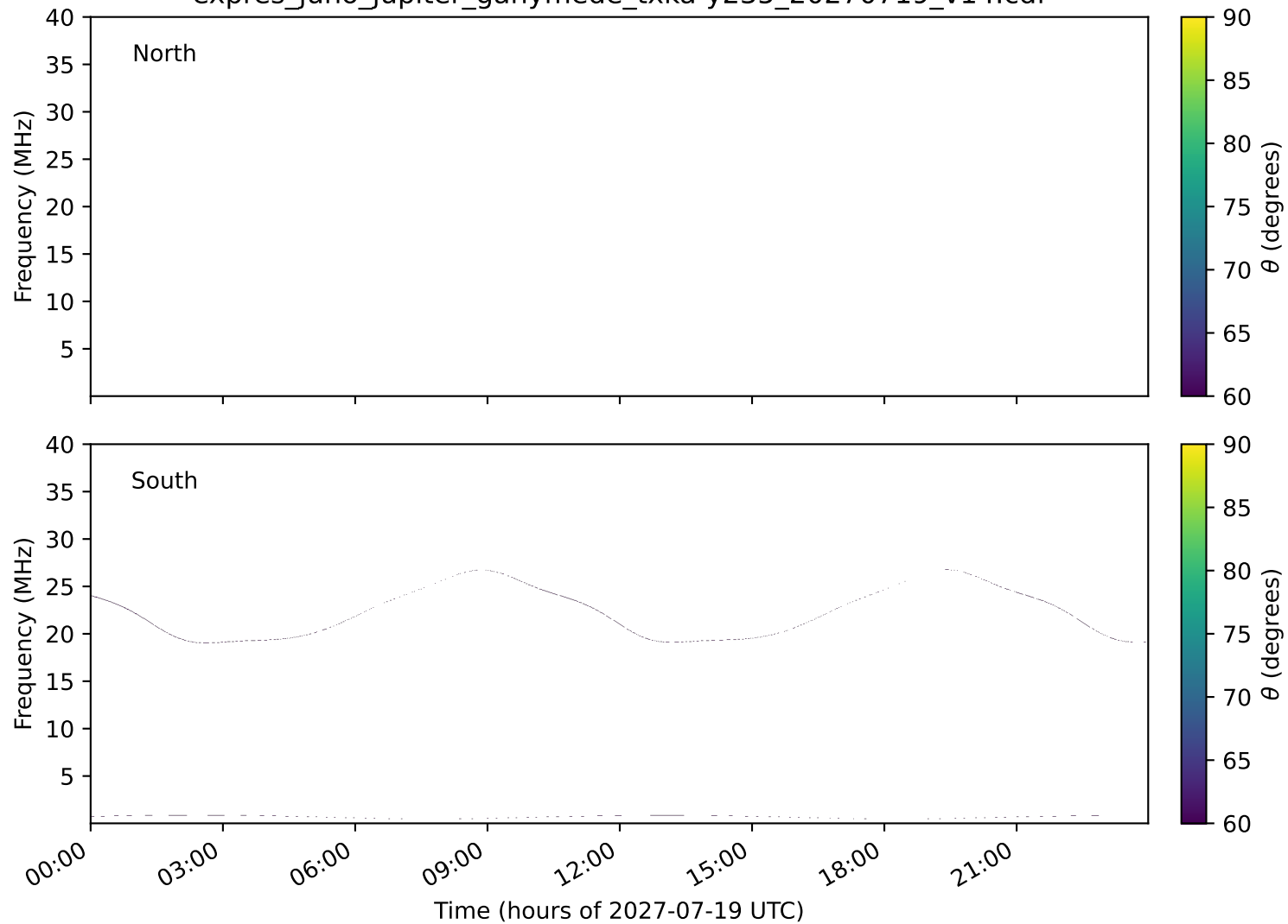
expres_juno_jupiter_ganymede_txka-y235_20270719_v14.cdf
