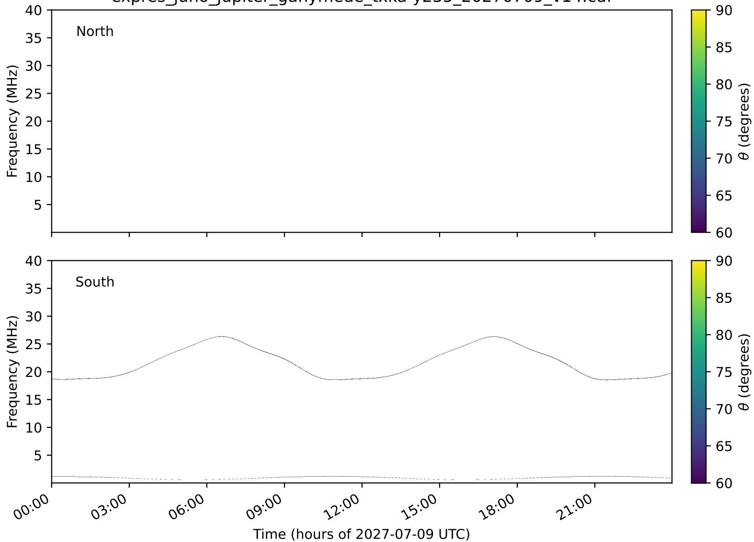
expres_juno_jupiter_ganymede_txka-y235_20270709_v14.cdf
