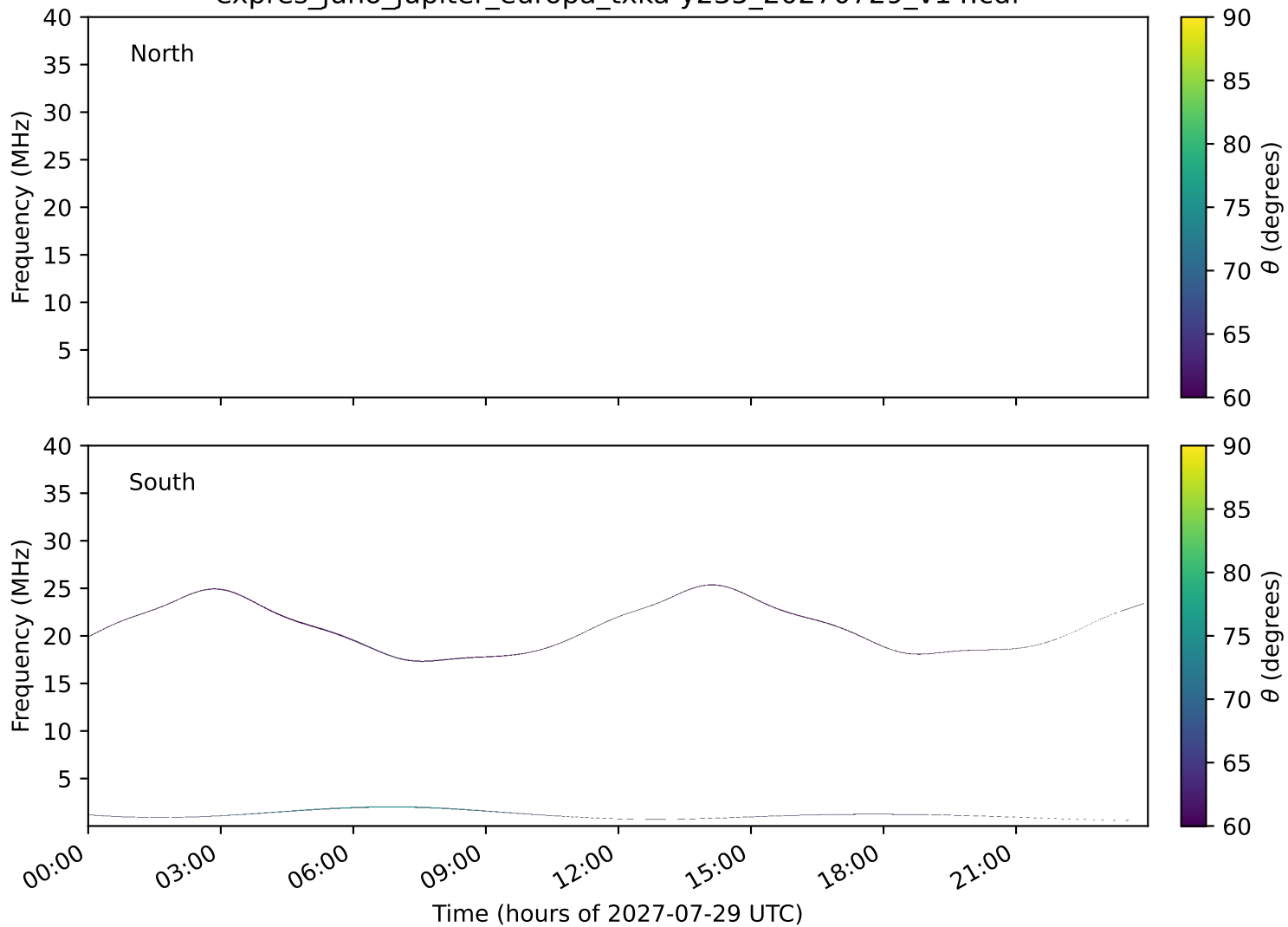
expres_juno_jupiter_europa_txka-y235_20270729_v14.cdf
