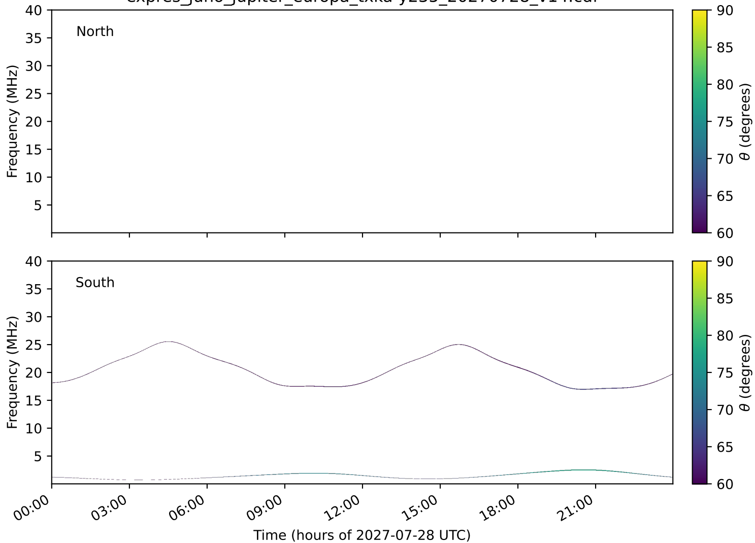
expres_juno_jupiter_europa_txka-y235_20270728_v14.cdf
