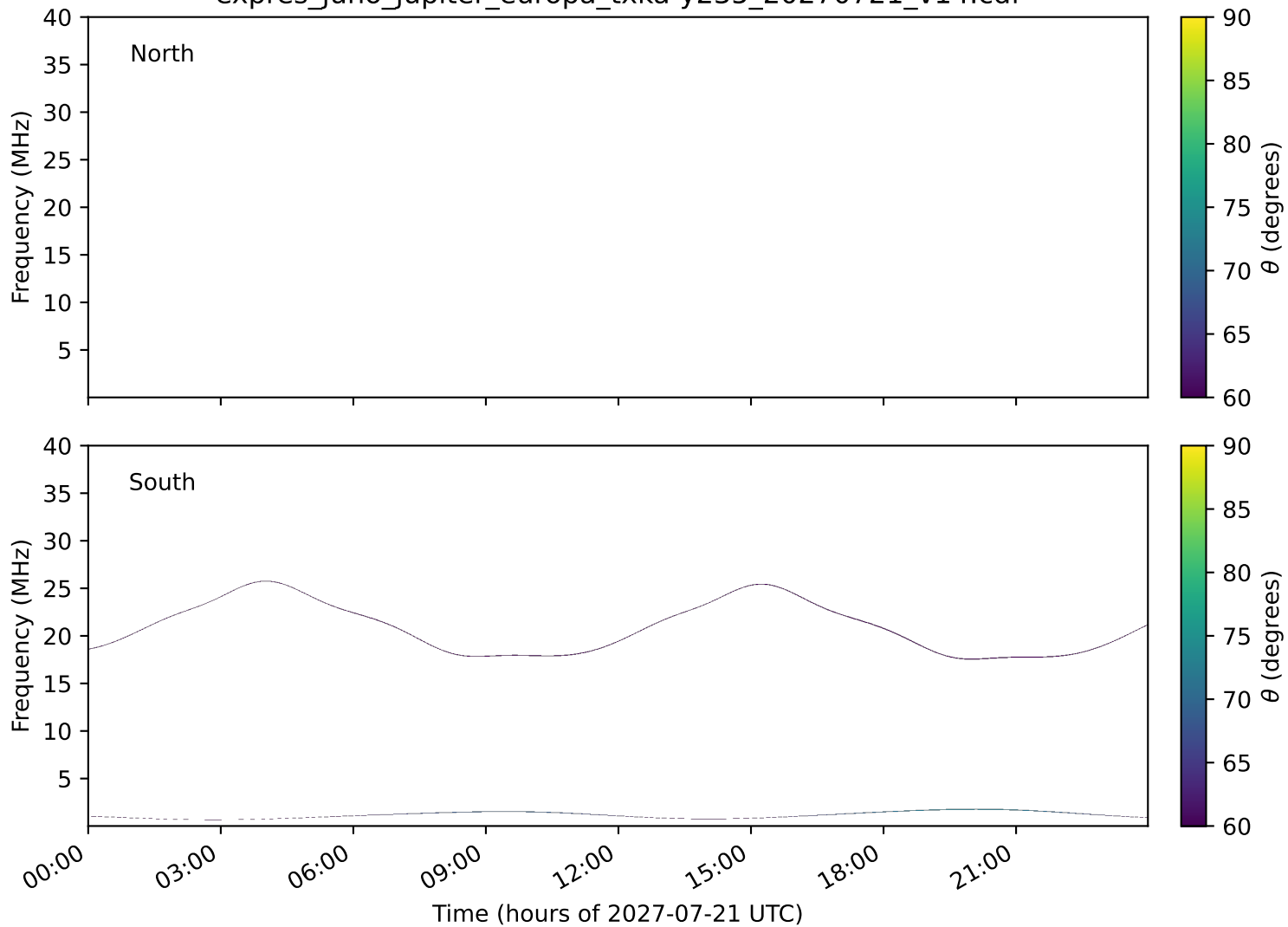
expres_juno_jupiter_europa_txka-y235_20270721_v14.cdf
