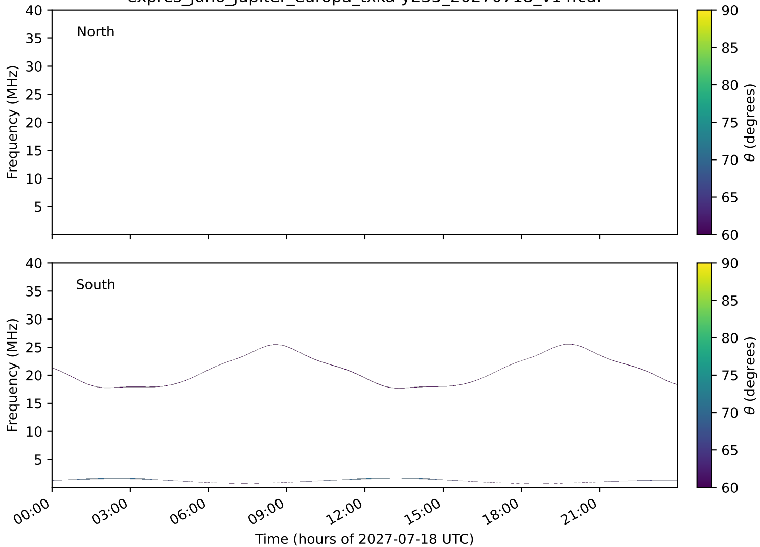
expres_juno_jupiter_europa_txka-y235_20270718_v14.cdf
