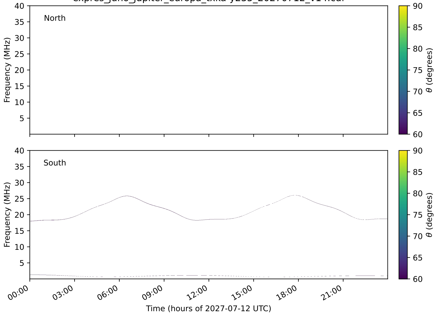
expres_juno_jupiter_europa_txka-y235_20270712_v14.cdf
