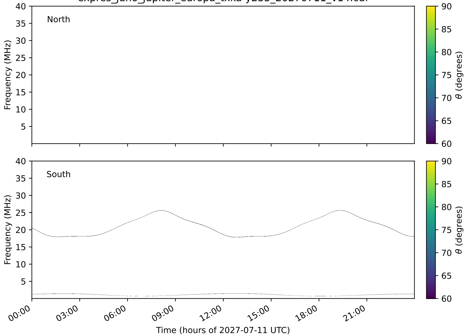
expres_juno_jupiter_europa_txka-y235_20270711_v14.cdf
