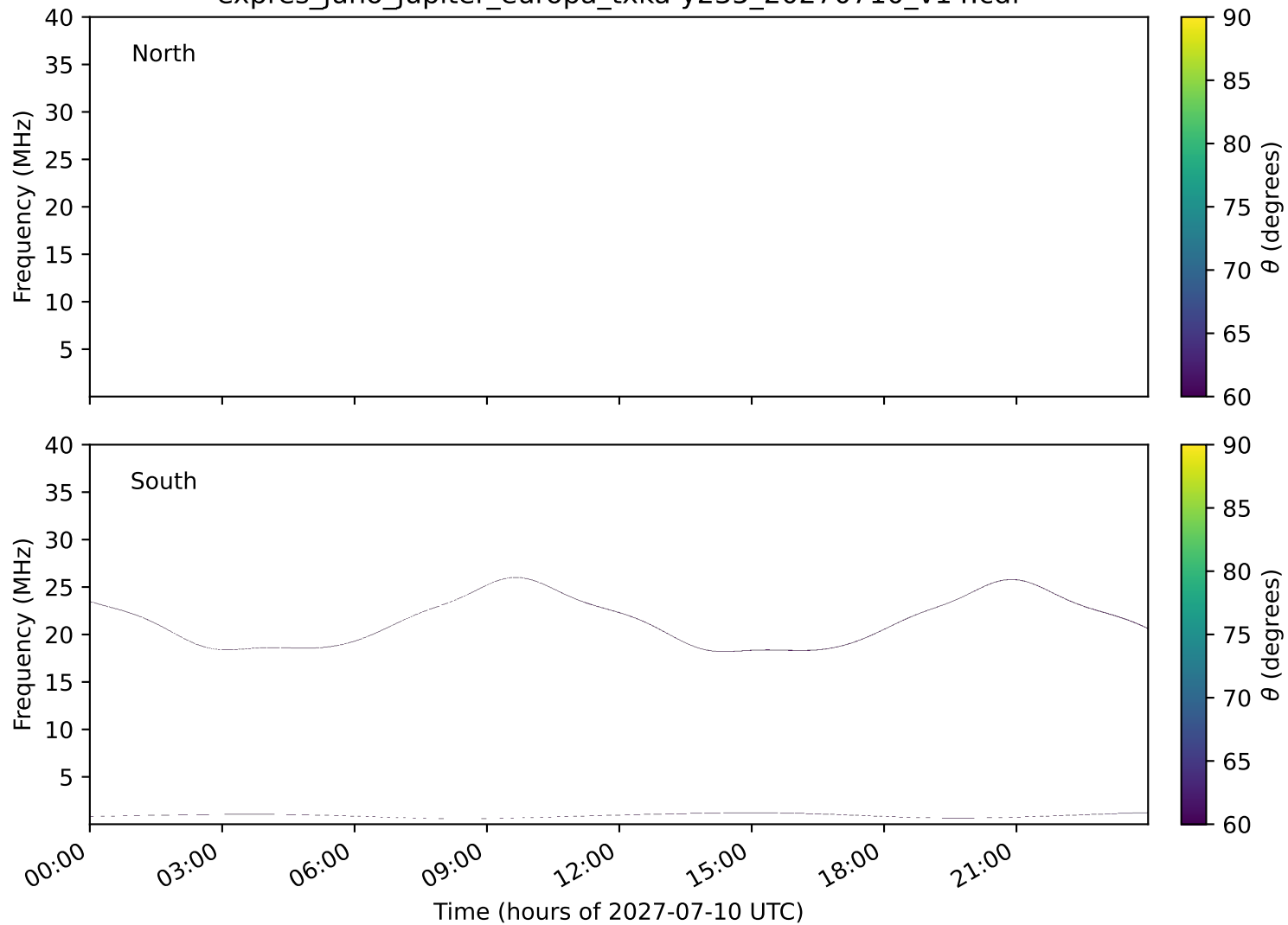
expres_juno_jupiter_europa_txka-y235_20270710_v14.cdf
