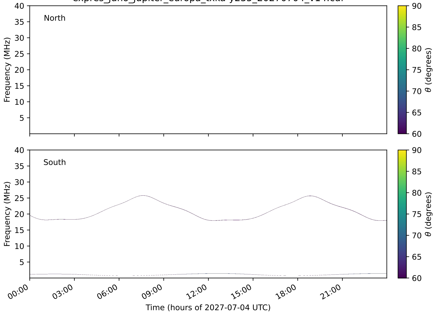
expres_juno_jupiter_europa_txka-y235_20270704_v14.cdf
