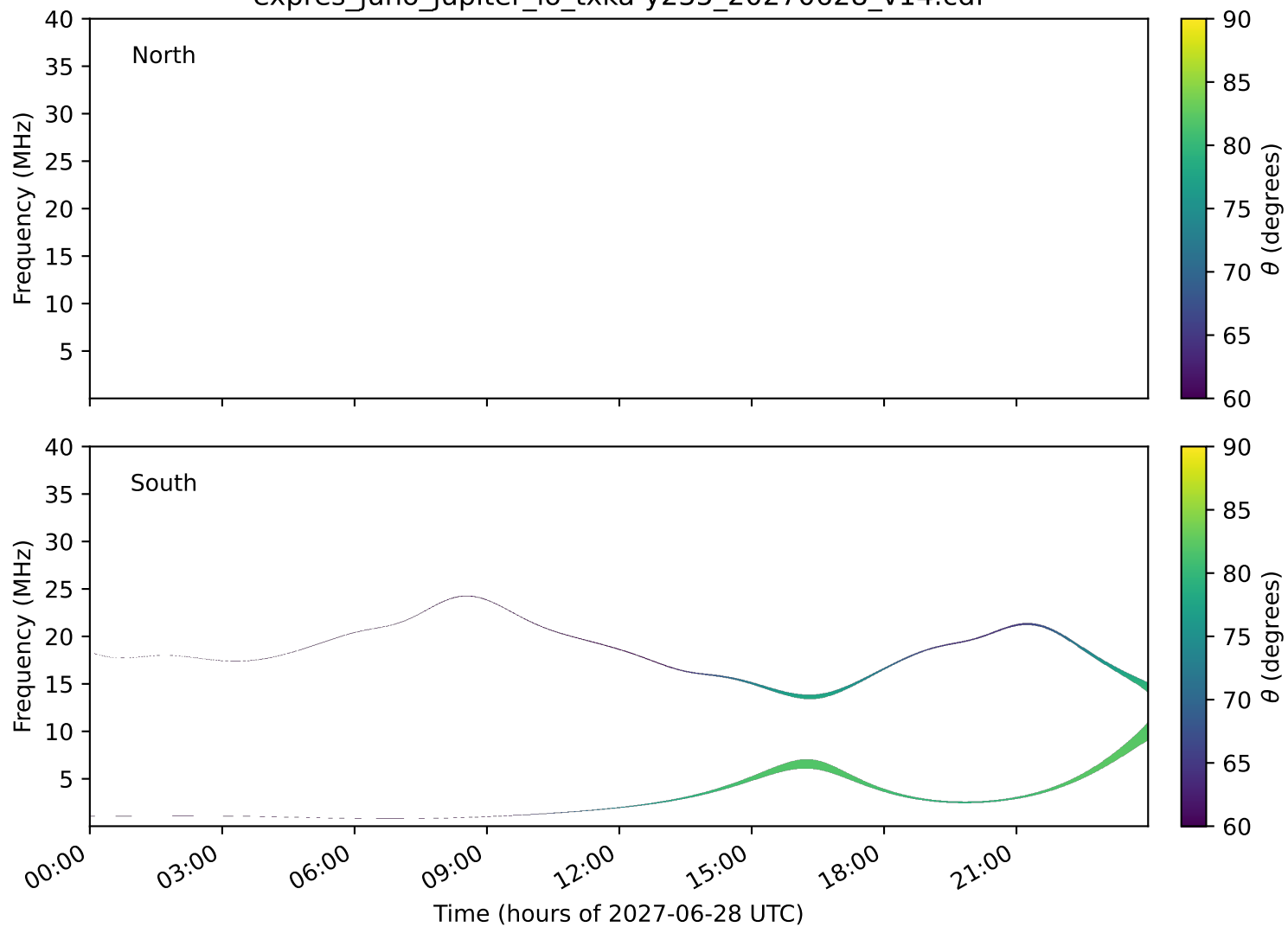
expres_juno_jupiter_io_txka-y235_20270628_v14.cdf
