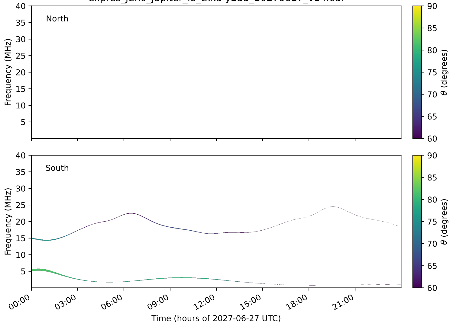
expres_juno_jupiter_io_txka-y235_20270627_v14.cdf
