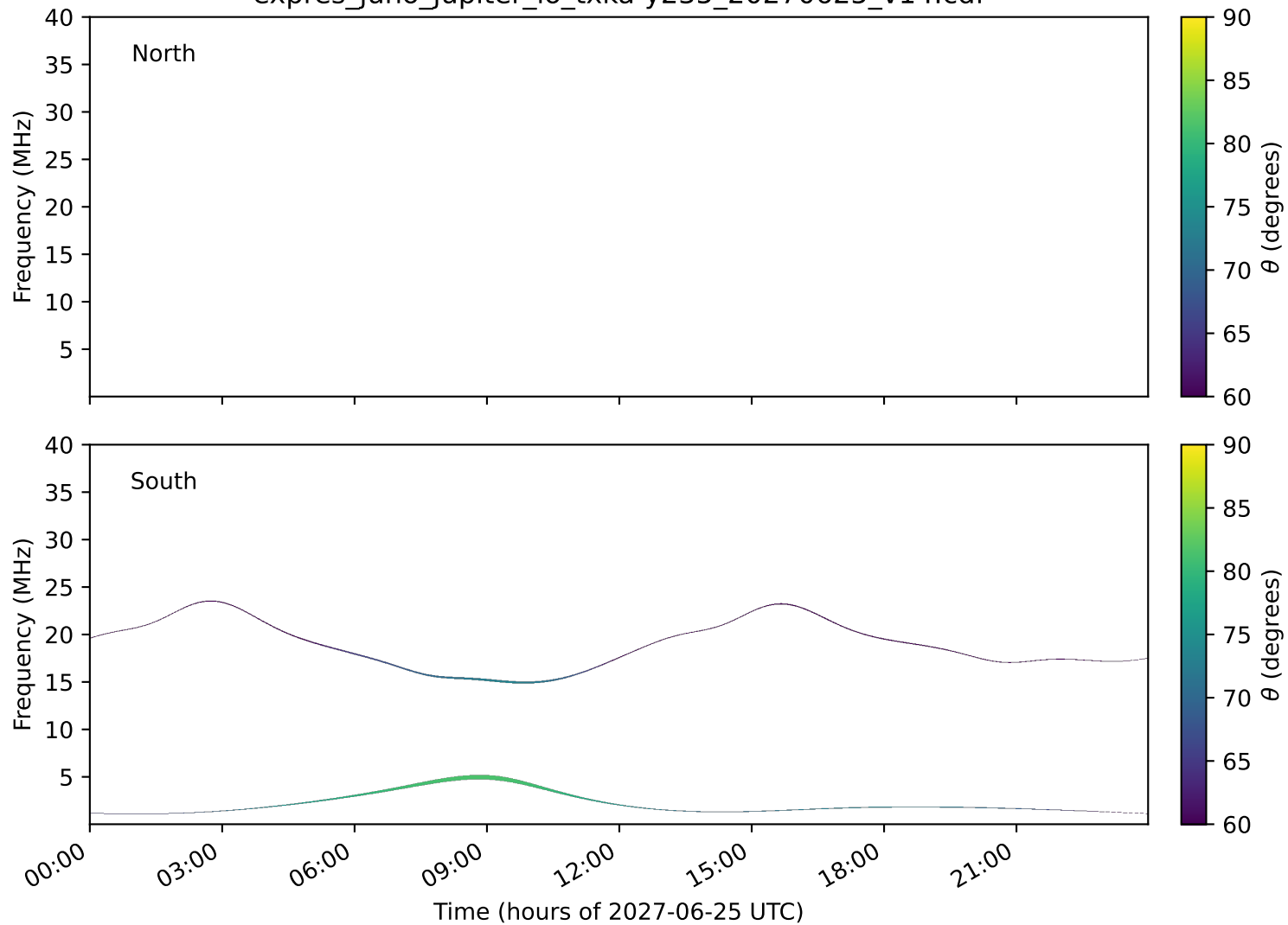
expres_juno_jupiter_io_txka-y235_20270625_v14.cdf
