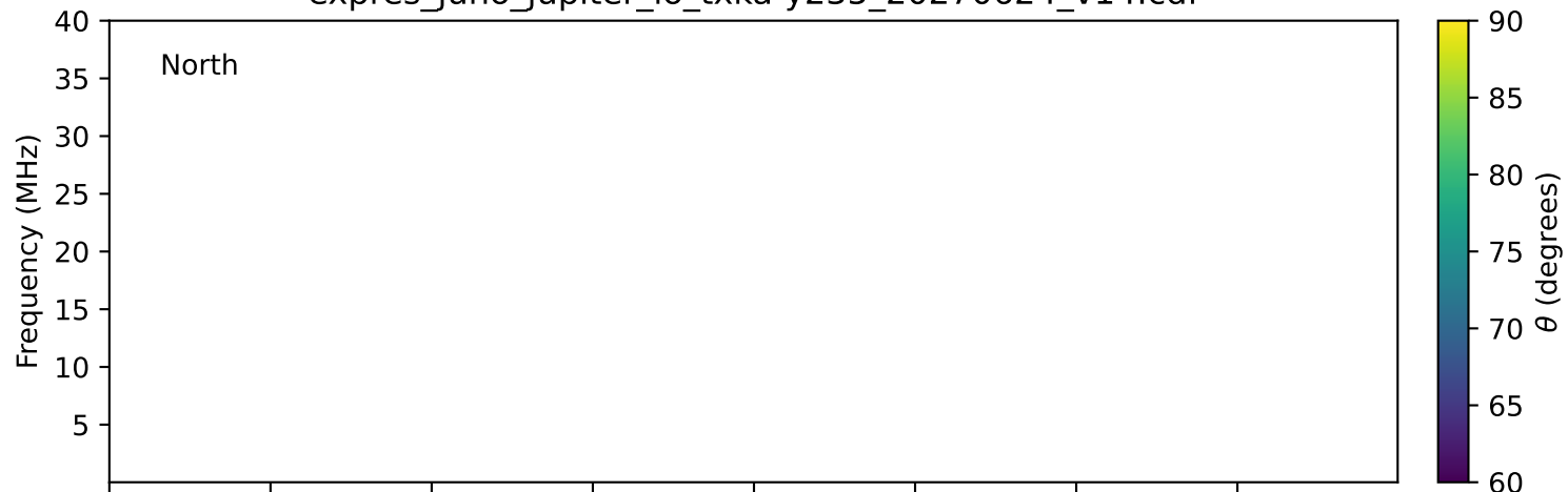
expres_juno_jupiter_io_txka-y235_20270624_v14.cdf
