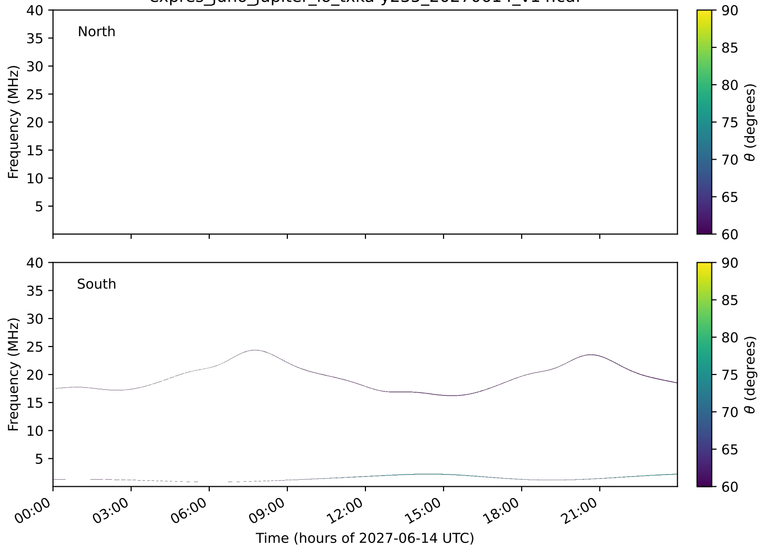
expres_juno_jupiter_io_txka-y235_20270614_v14.cdf
