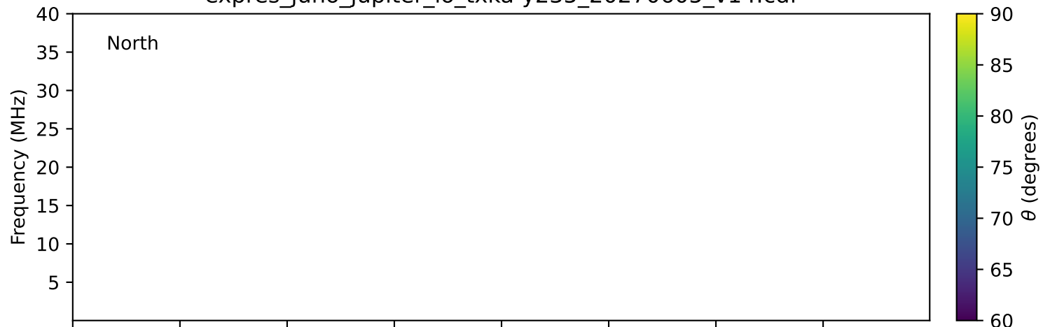
expres_juno_jupiter_io_txka-y235_20270605_v14.cdf
