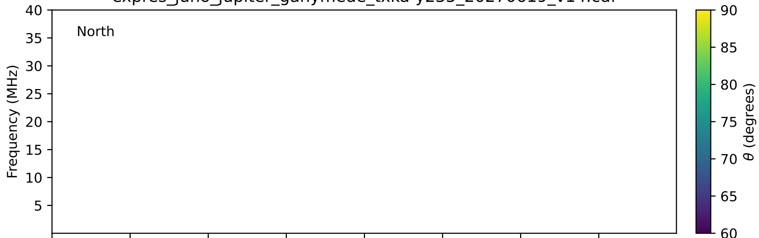
expres_juno_jupiter_ganymede_txka-y235_20270619_v14.cdf
