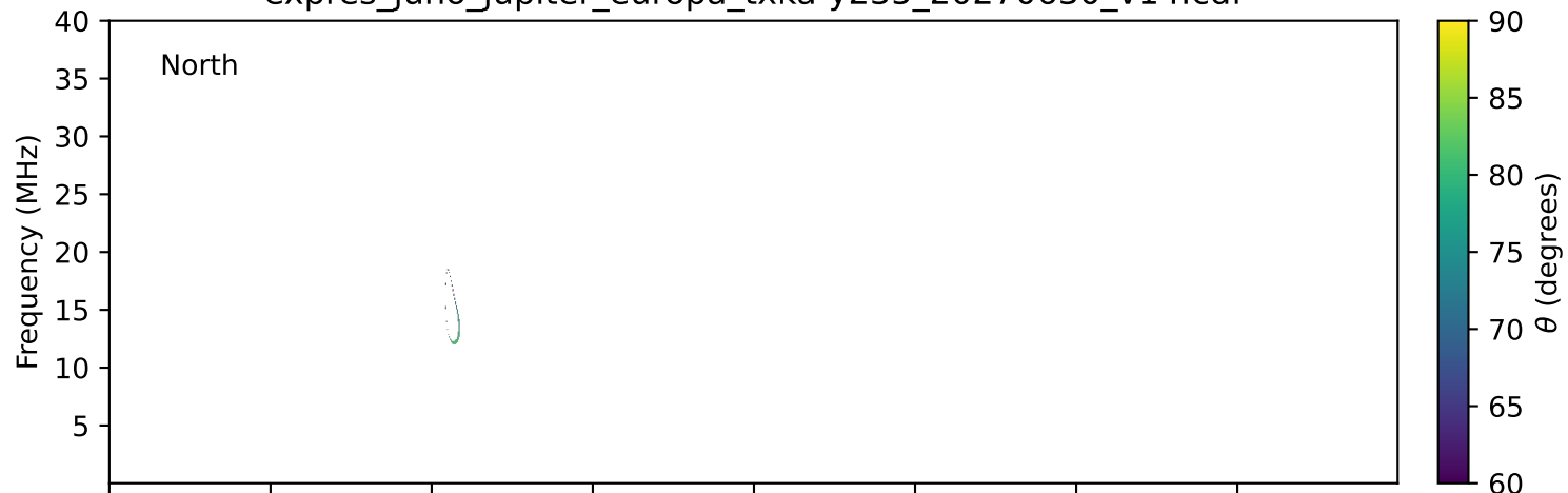
expres_juno_jupiter_europa_txka-y235_20270630_v14.cdf
