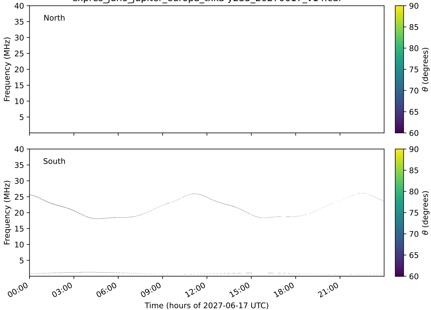
expres_juno_jupiter_europa_txka-y235_20270617_v14.cdf
