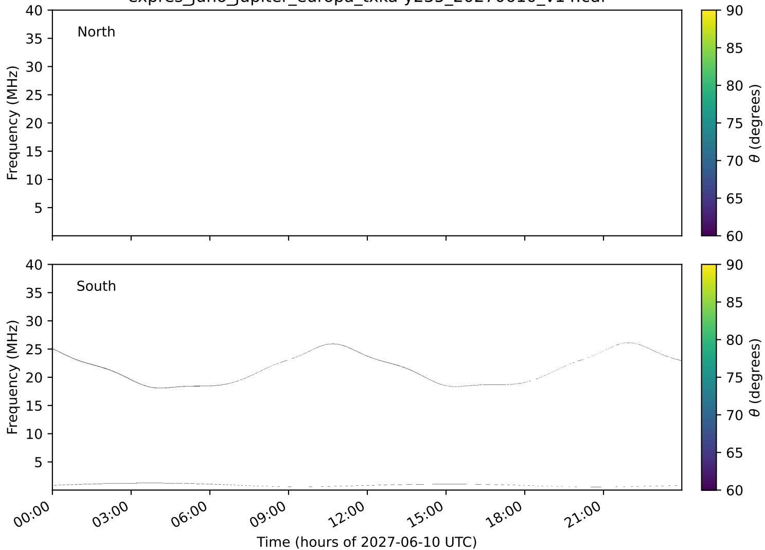
expres_juno_jupiter_europa_txka-y235_20270610_v14.cdf
