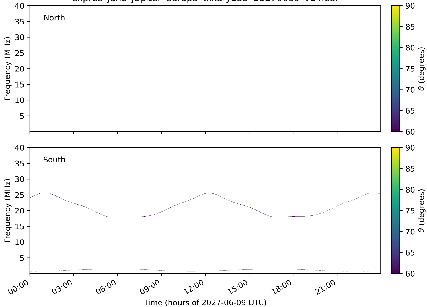
expres_juno_jupiter_europa_txka-y235_20270609_v14.cdf
