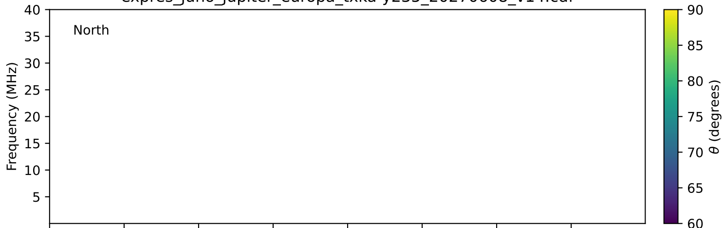
expres_juno_jupiter_europa_txka-y235_20270608_v14.cdf
