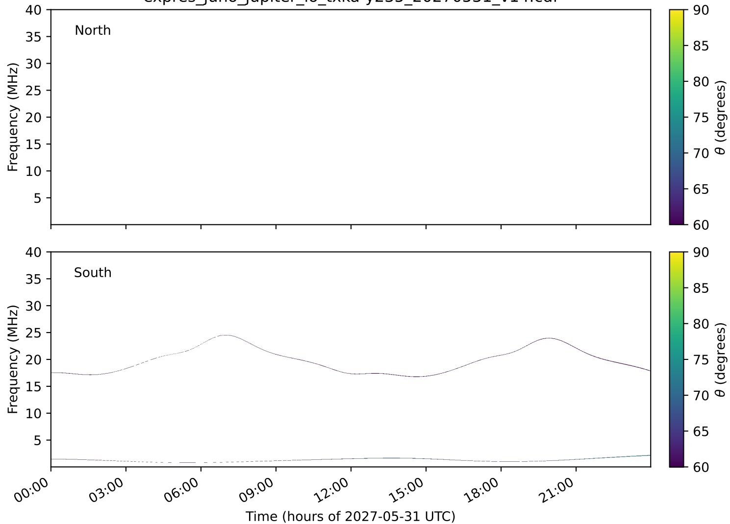
expres_juno_jupiter_io_txka-y235_20270531_v14.cdf
