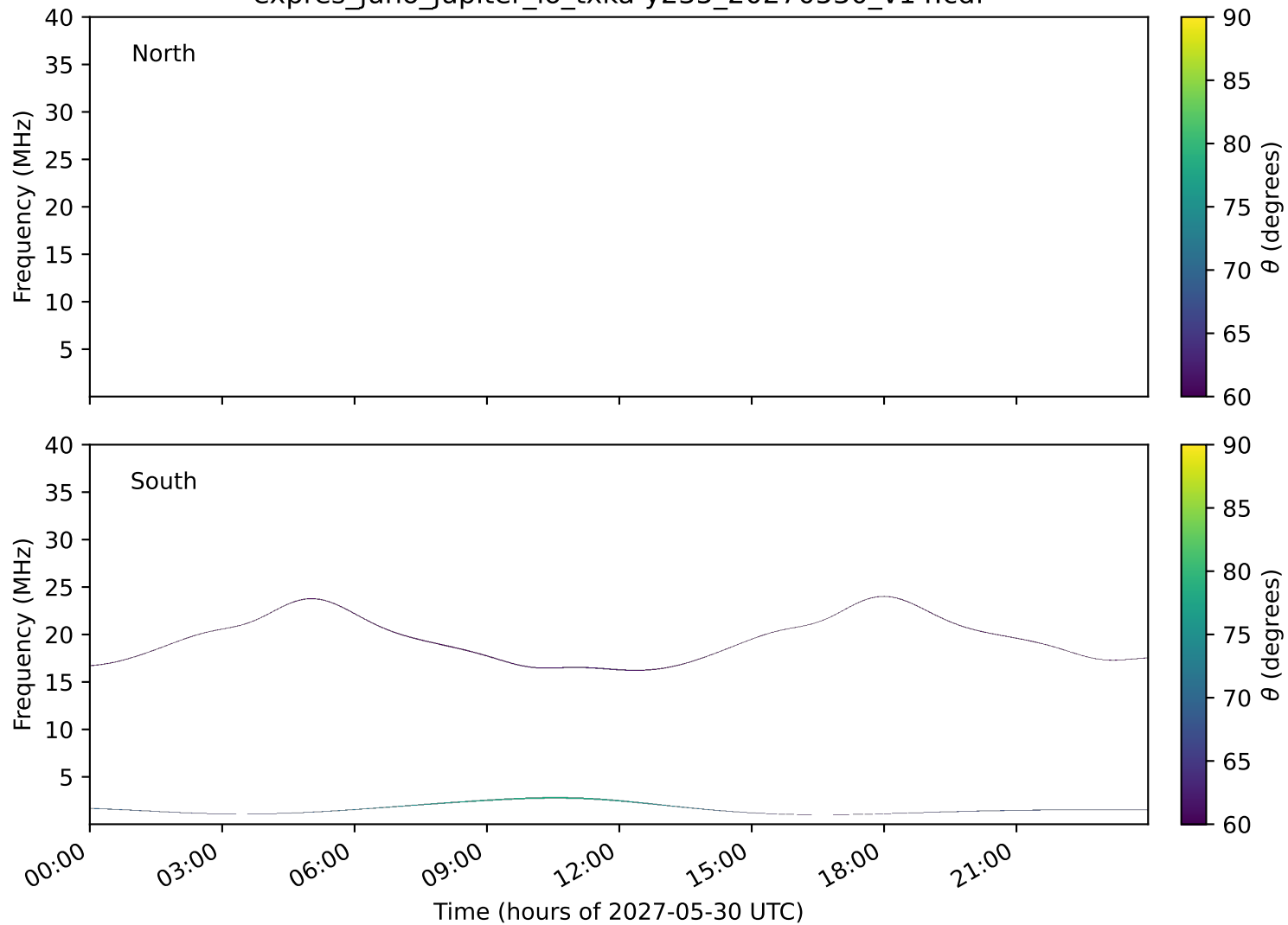
expres_juno_jupiter_io_txka-y235_20270530_v14.cdf
