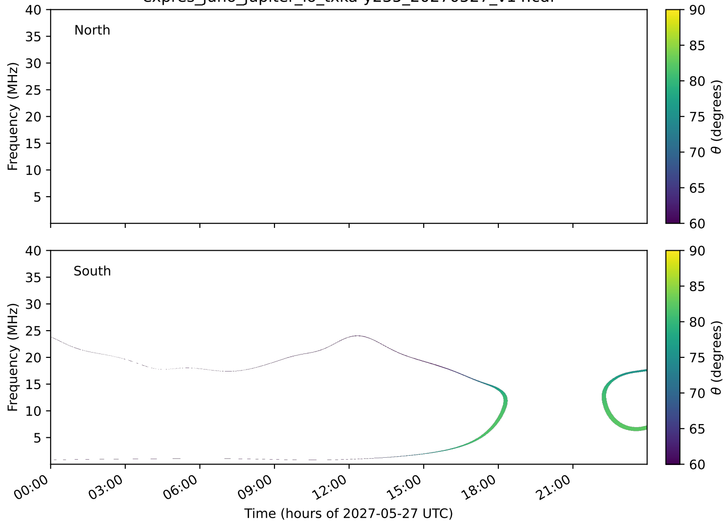
expres_juno_jupiter_io_txka-y235_20270527_v14.cdf
