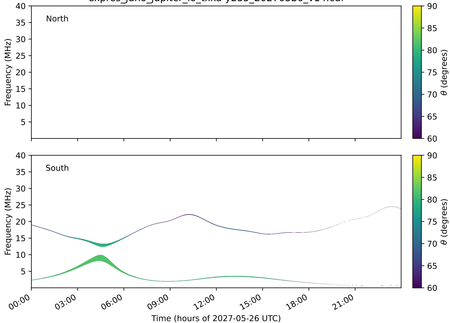
expres_juno_jupiter_io_txka-y235_20270526_v14.cdf
