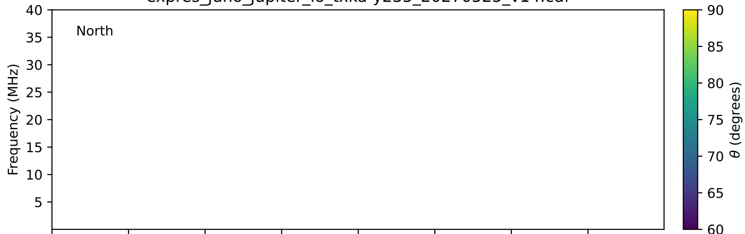
expres_juno_jupiter_io_txka-y235_20270525_v14.cdf
