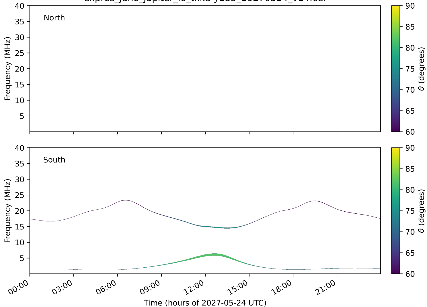
expres_juno_jupiter_io_txka-y235_20270524_v14.cdf
