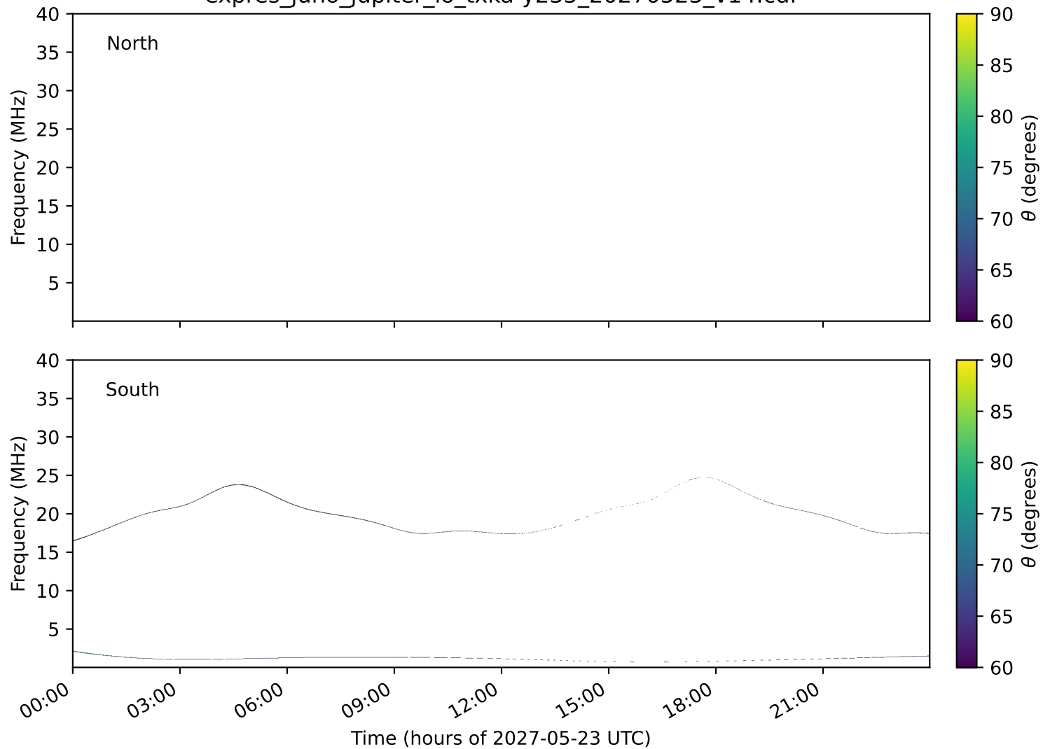
expres_juno_jupiter_io_txka-y235_20270523_v14.cdf
