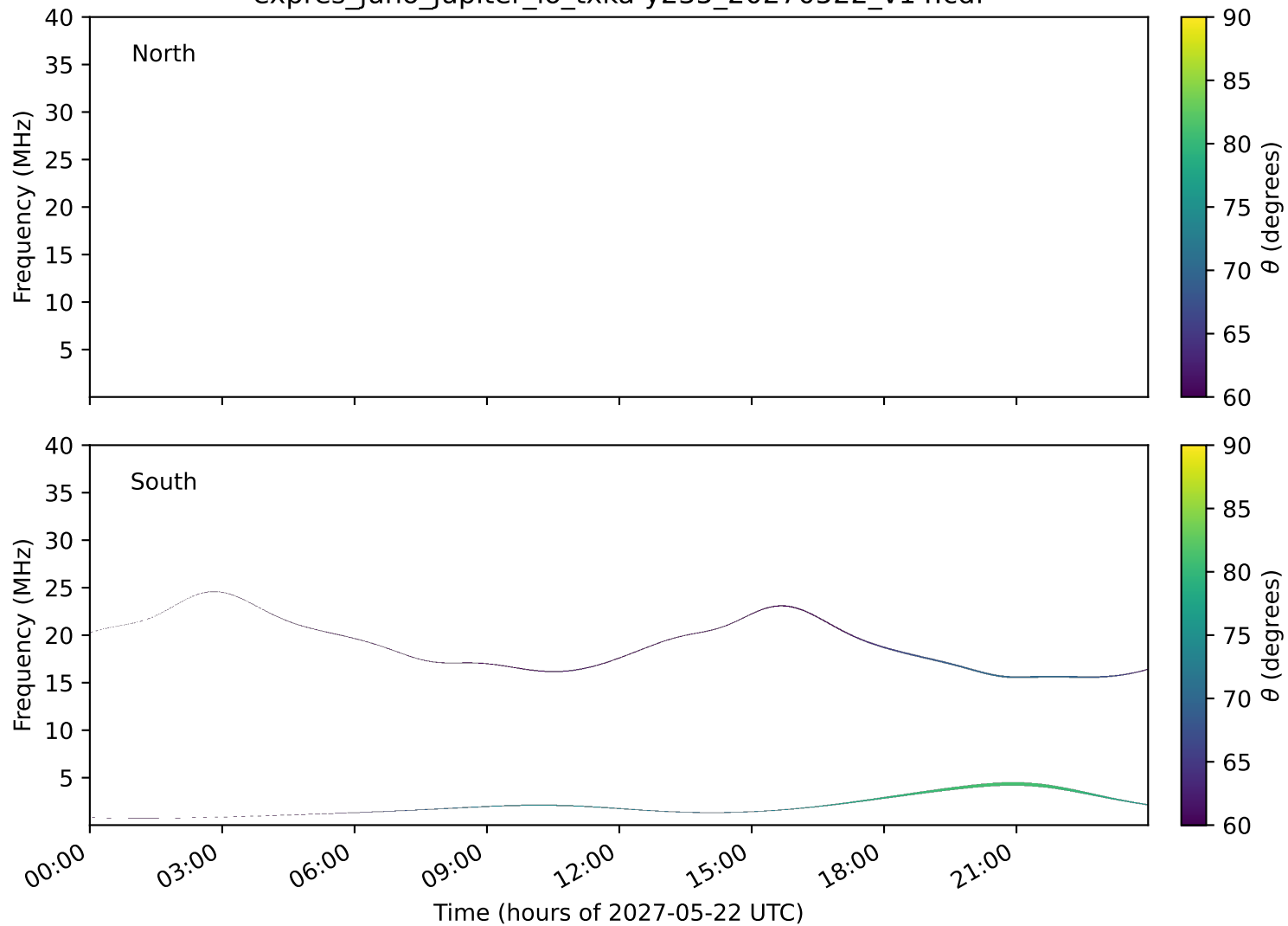
expres_juno_jupiter_io_txka-y235_20270522_v14.cdf
