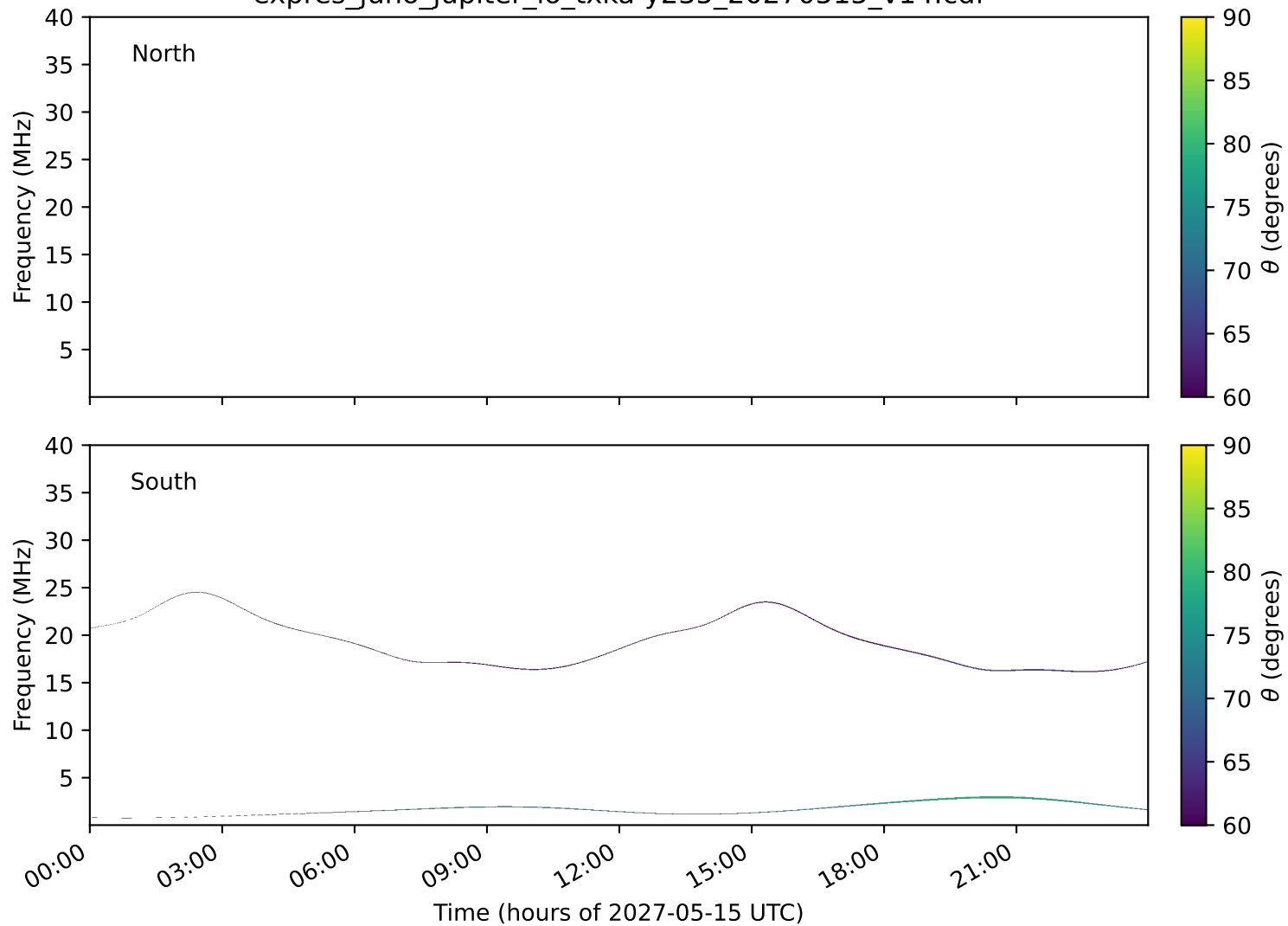
expres_juno_jupiter_io_txka-y235_20270515_v14.cdf
