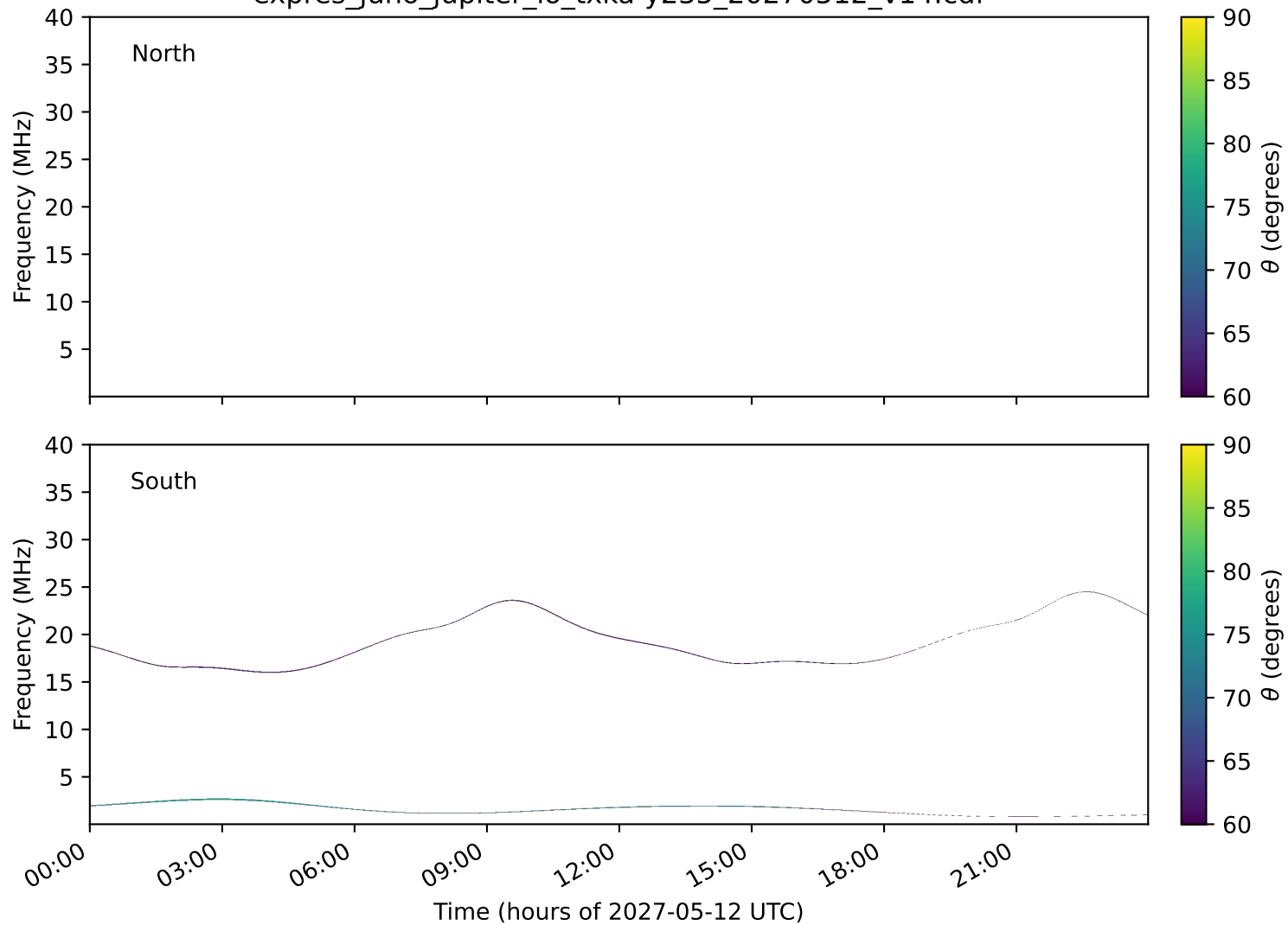
expres_juno_jupiter_io_txka-y235_20270512_v14.cdf
