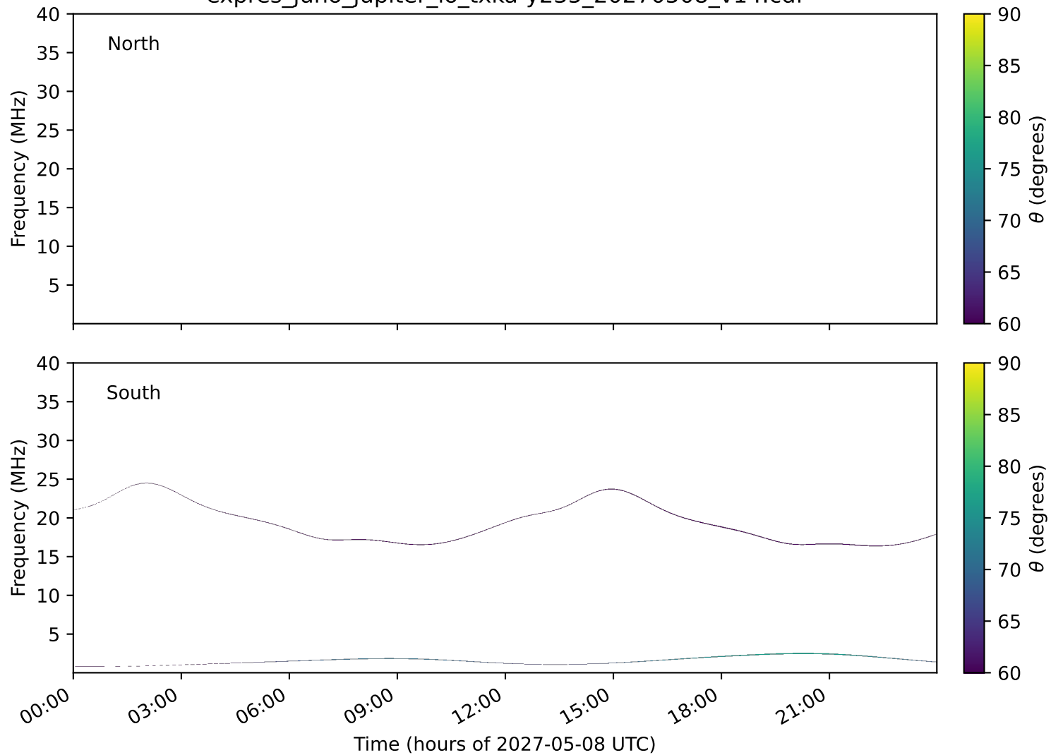
expres_juno_jupiter_io_txka-y235_20270508_v14.cdf
