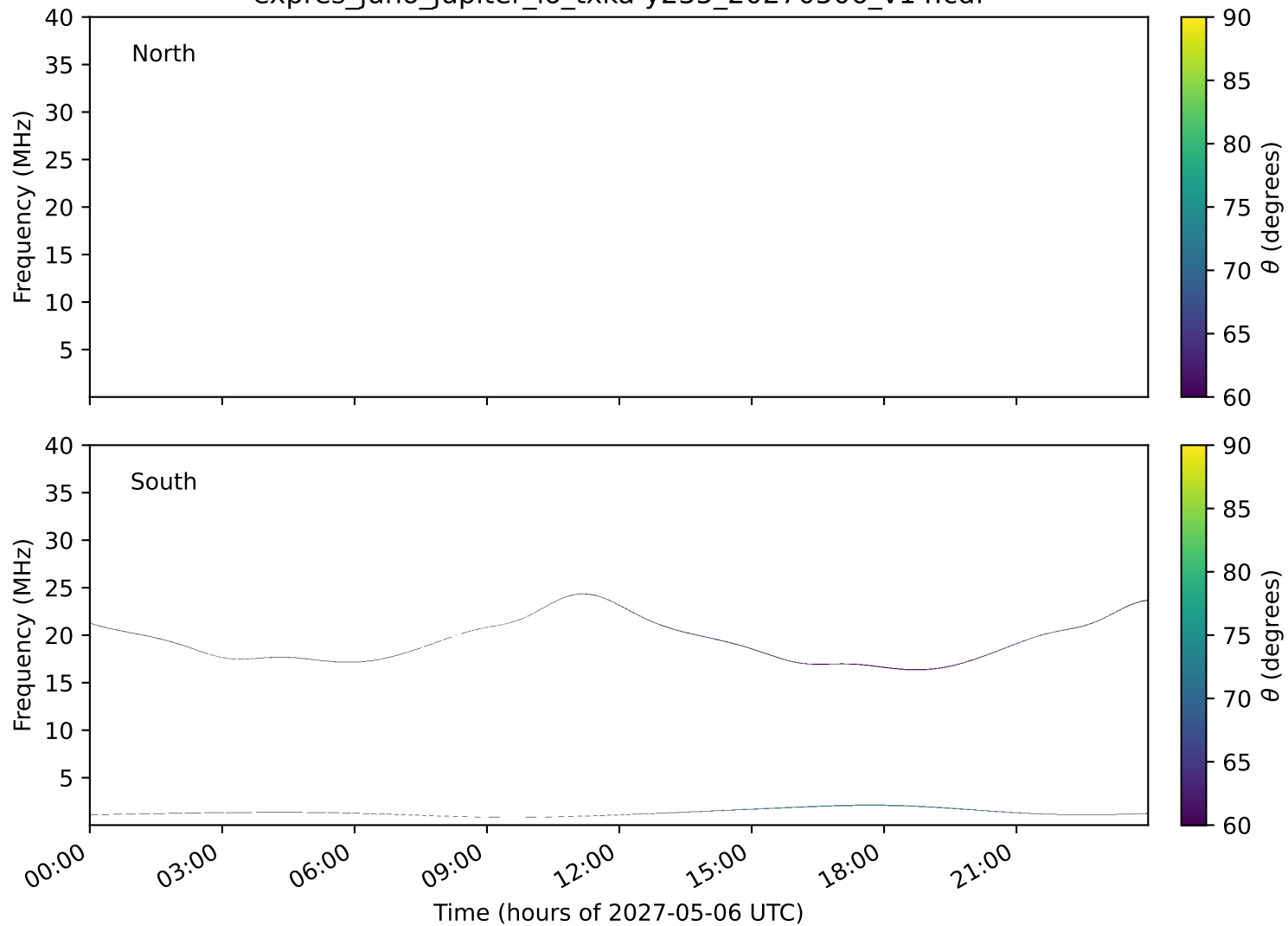
expres_juno_jupiter_io_txka-y235_20270506_v14.cdf
