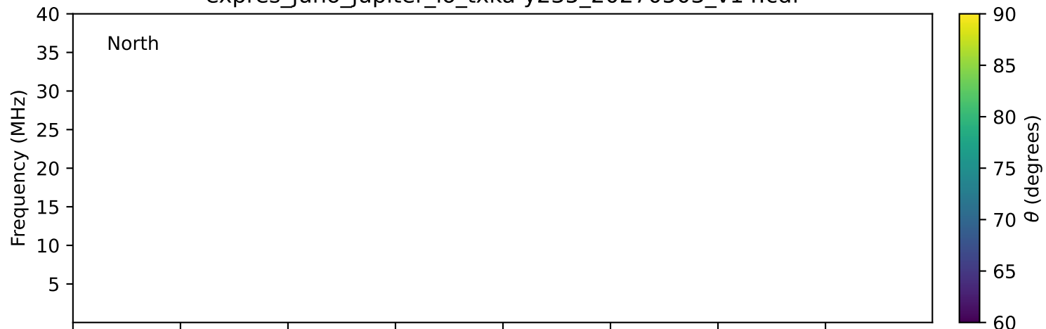
expres_juno_jupiter_io_txka-y235_20270503_v14.cdf
