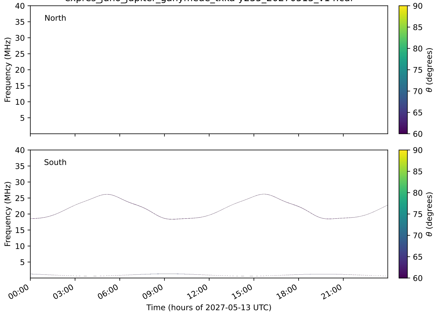
expres_juno_jupiter_ganymede_txka-y235_20270513_v14.cdf
