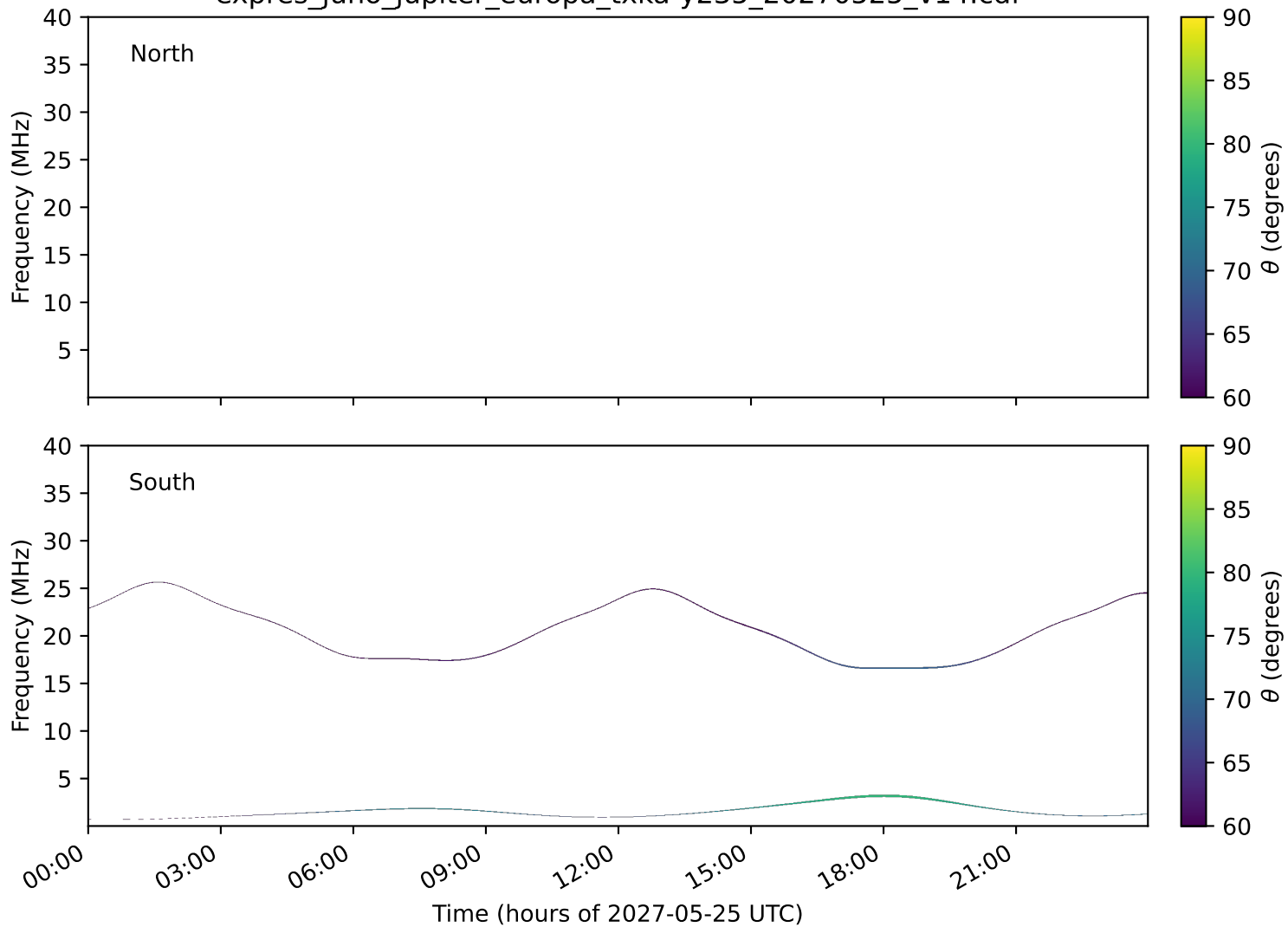
expres_juno_jupiter_europa_txka-y235_20270525_v14.cdf
