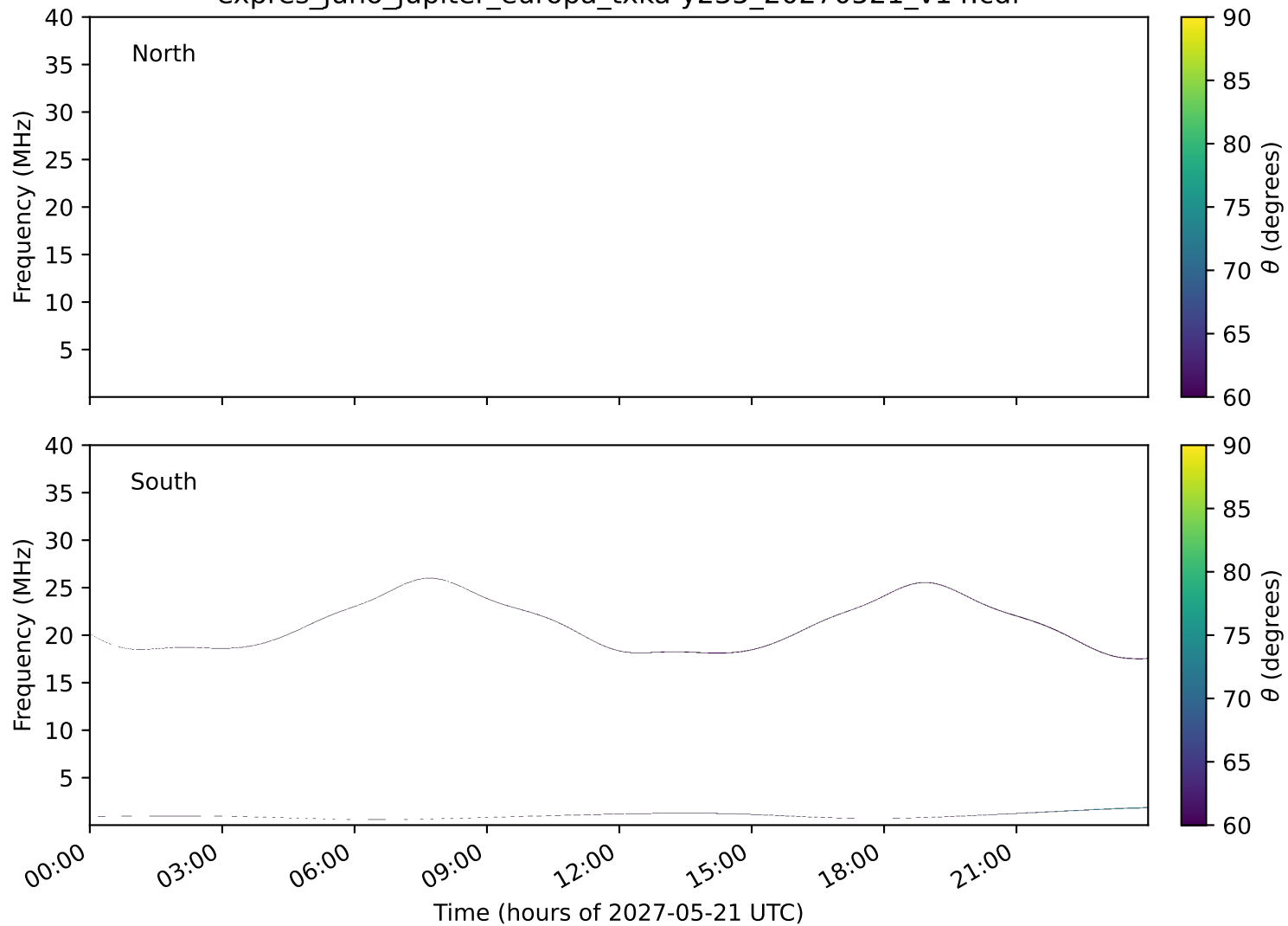
expres_juno_jupiter_europa_txka-y235_20270521_v14.cdf
