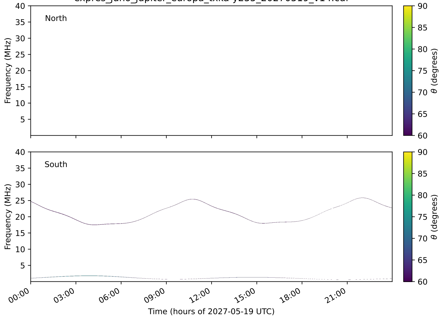
expres_juno_jupiter_europa_txka-y235_20270519_v14.cdf
