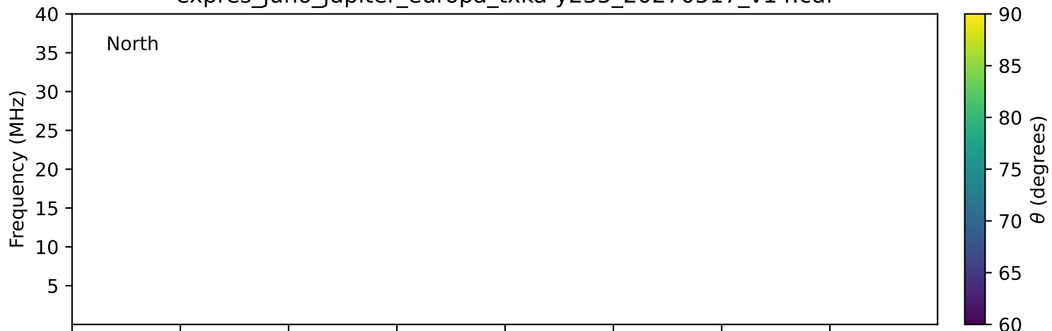
expres_juno_jupiter_europa_txka-y235_20270517_v14.cdf
