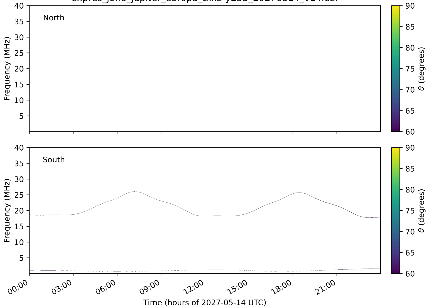
expres_juno_jupiter_europa_txka-y235_20270514_v14.cdf
