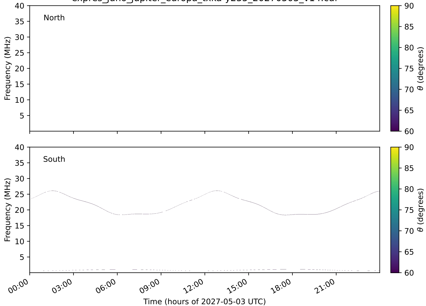
expres_juno_jupiter_europa_txka-y235_20270503_v14.cdf
