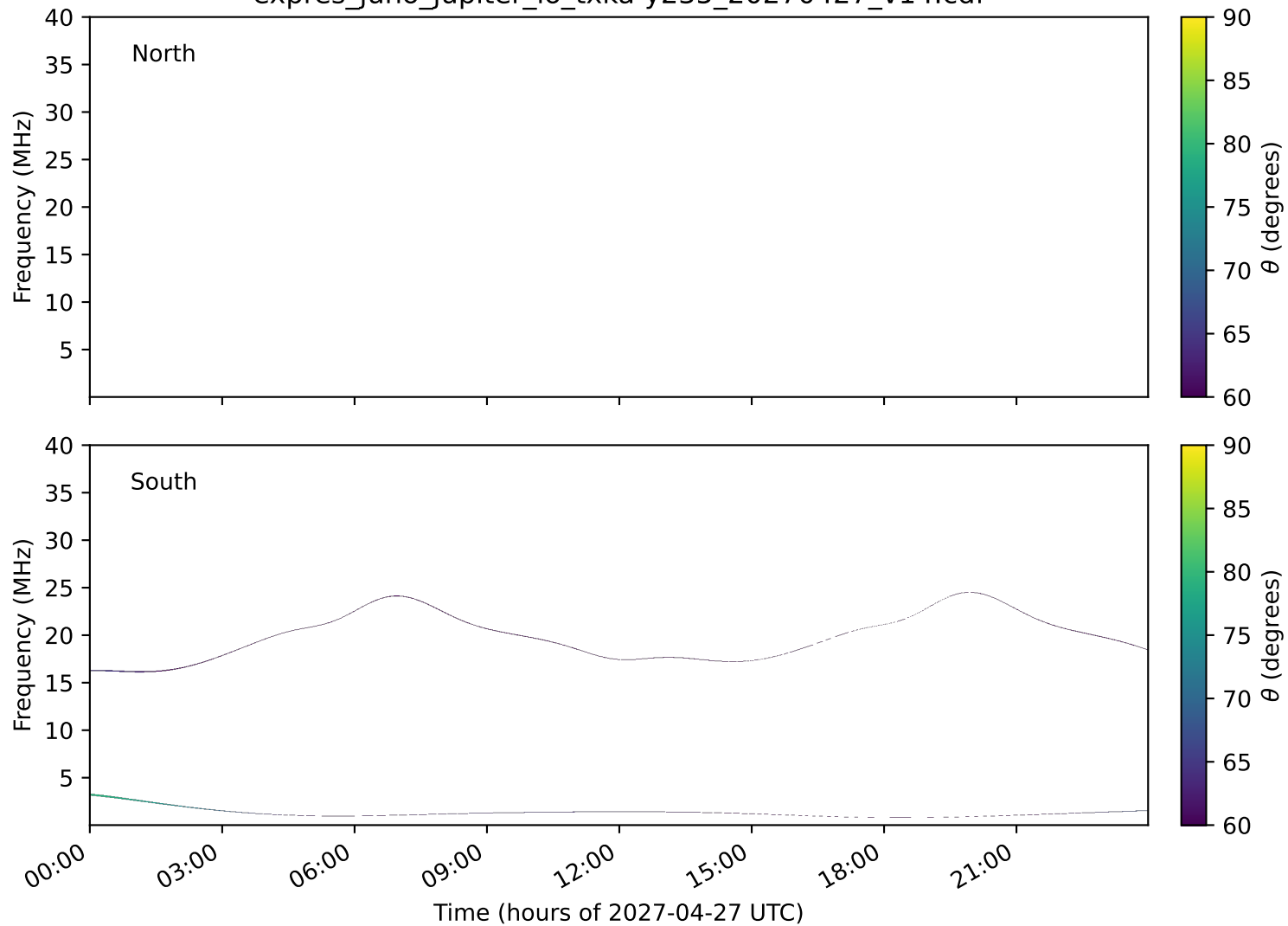
expres_juno_jupiter_io_txka-y235_20270427_v14.cdf
