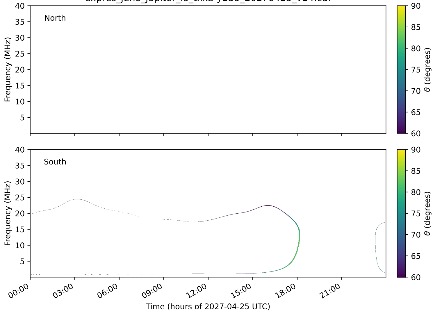
expres_juno_jupiter_io_txka-y235_20270425_v14.cdf
