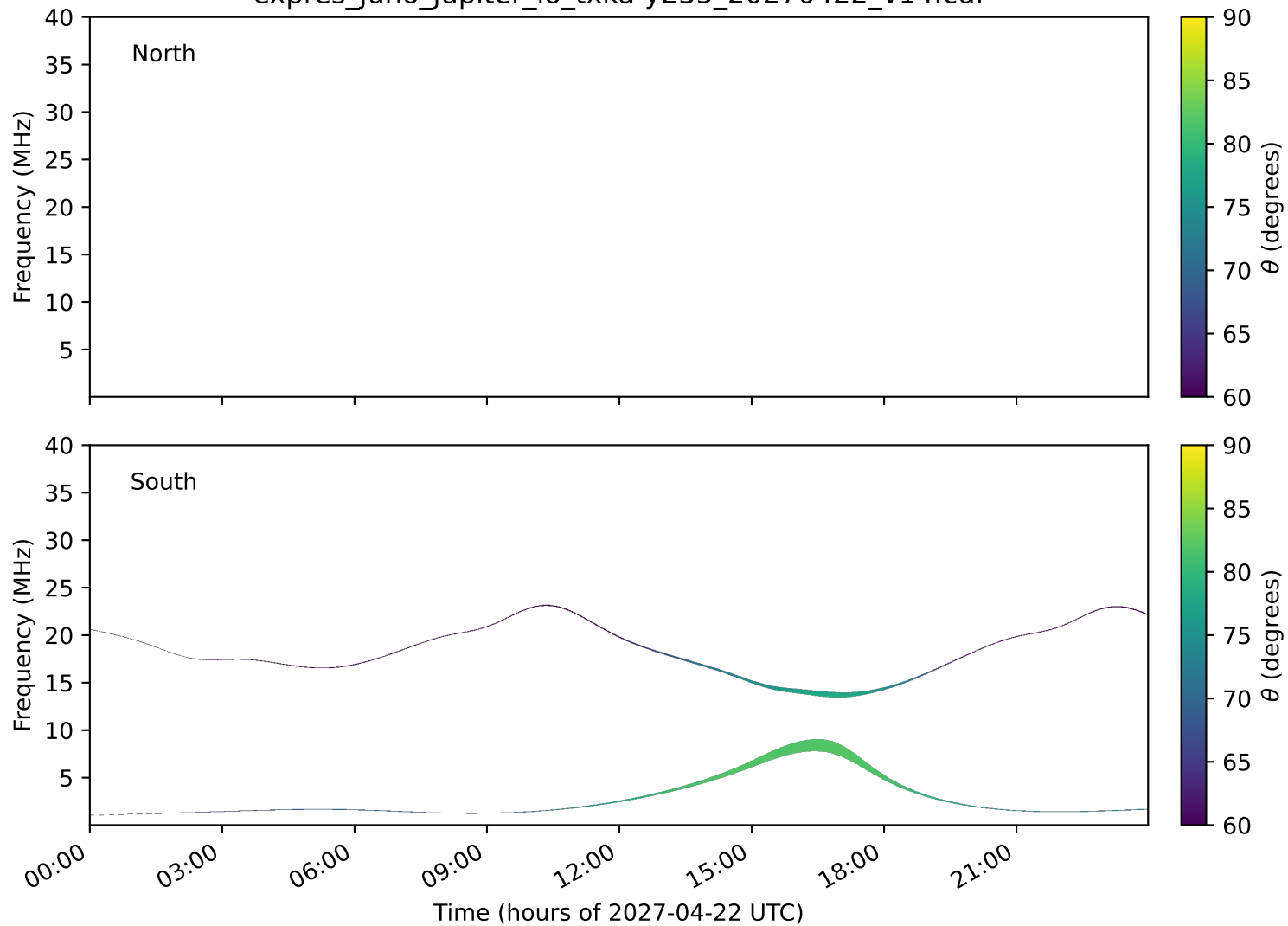
expres_juno_jupiter_io_txka-y235_20270422_v14.cdf
