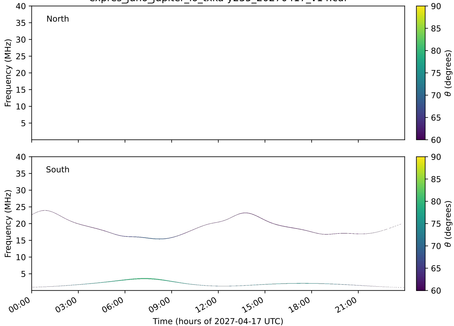
expres_juno_jupiter_io_txka-y235_20270417_v14.cdf
