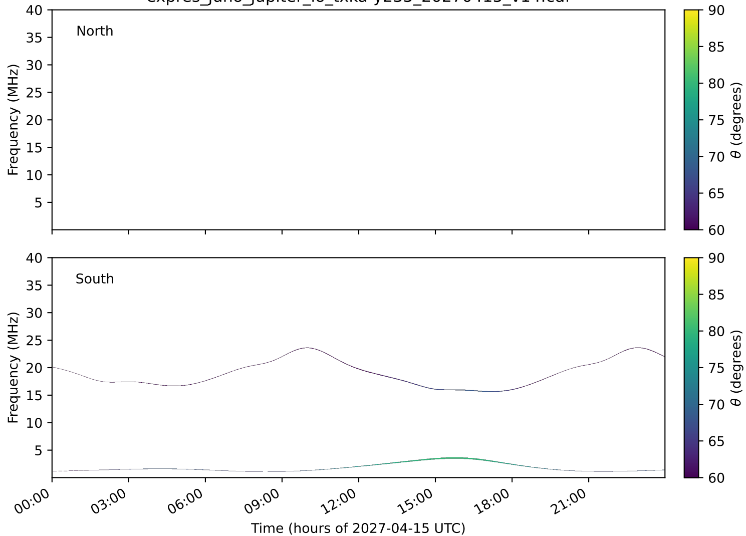
expres_juno_jupiter_io_txka-y235_20270415_v14.cdf
